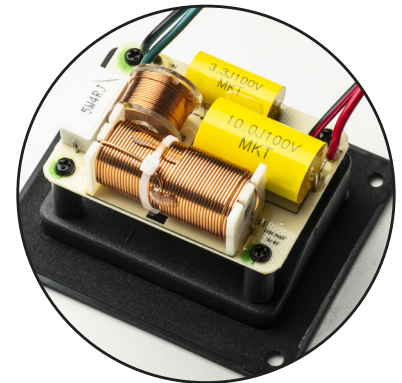
2-way cross-over
